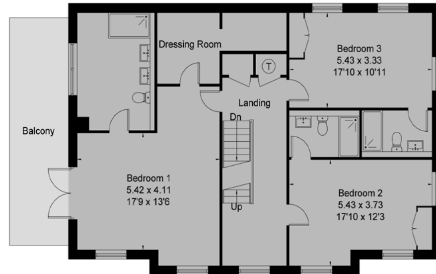
First Floor
